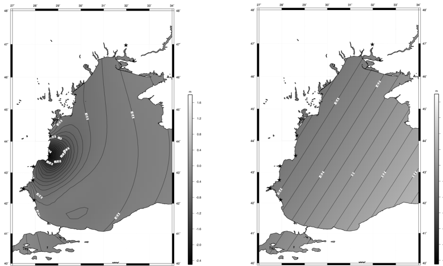
Fig. 6: 2 nd order (left) and 1 st order (right) corrector surfaces between gravimetric quasi-geoid heights and altimetric geoid heights.
