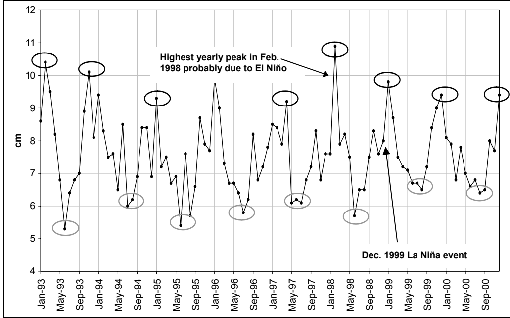
Fig. 4: Sea level variations between 1993 and 2001.
