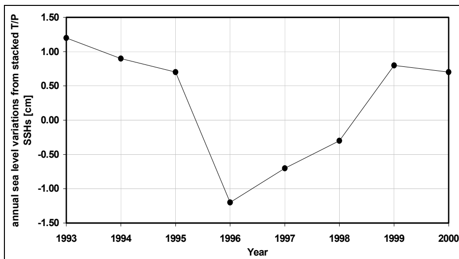
Fig. 3: Annual sea level variations from T/P SSHs.
